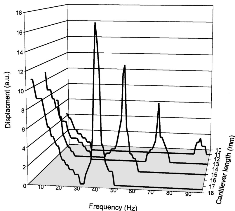
FIG. 10. SWNT/naftion/SWNT cantilever displacement at an ac bias of 3.5 V as a function of the frequency at different cantilever lengths.
